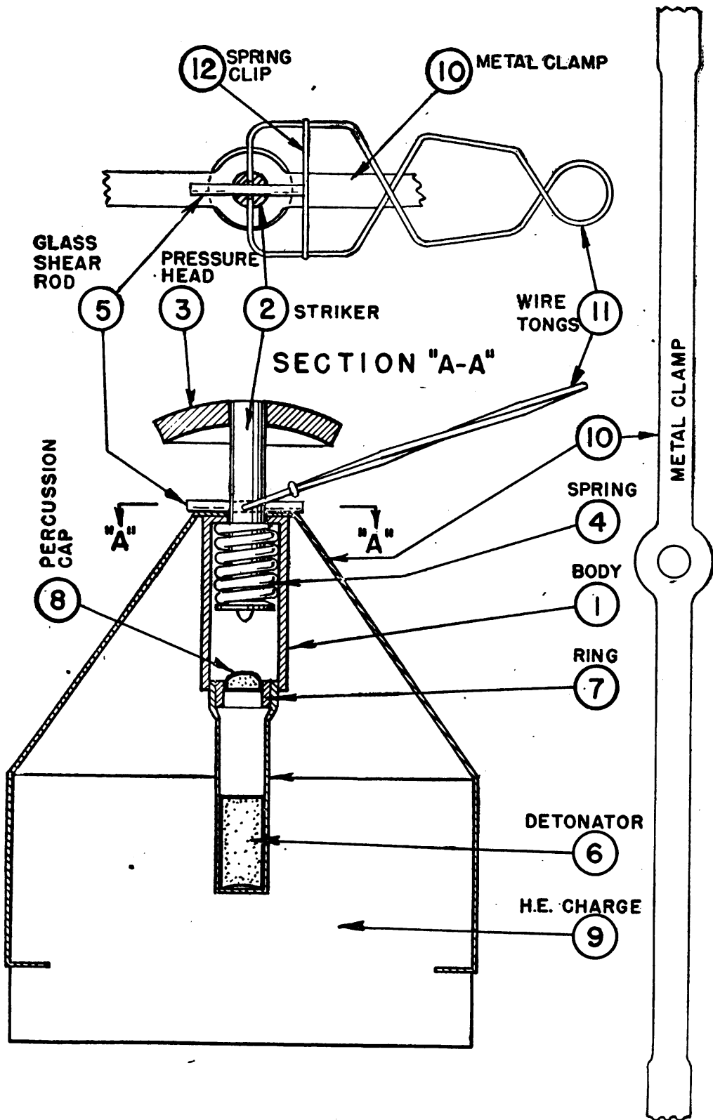
FIGURE 14.2.—Weissman igniter.
